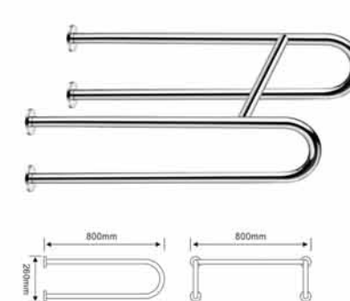
YX-3336 Material : SUS 304 Size(mm) : 800x800x260 Finish : Matt / Polish
