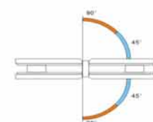
YX-2017C 180° 缓冲阻尼玻璃夹 180° Hydraulic Glass Clamp
